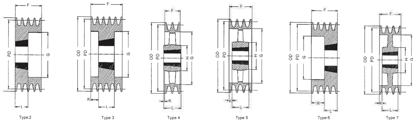
Pulley Groove Dimensions (ISO Standard)
